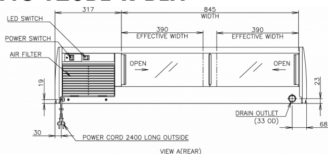
VIEW A(REAR)
