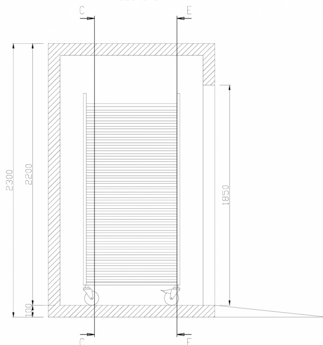
SEC B-B
